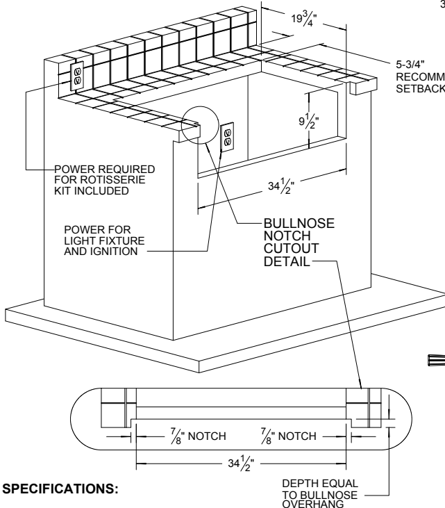
TYPICAL ARTP-36 INSTALLATION
