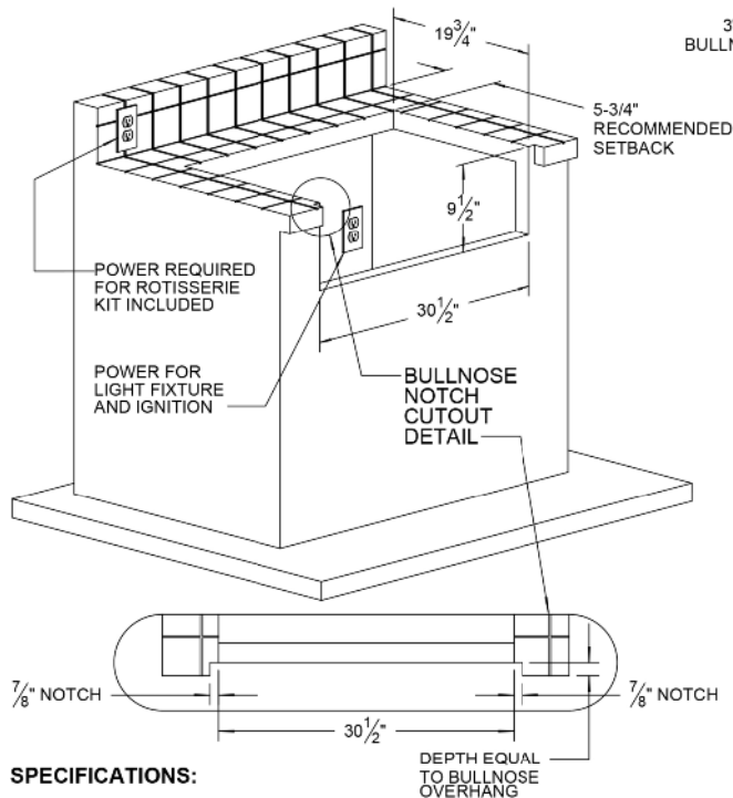
TYPICAL ARTP-32 INSTALLATION
