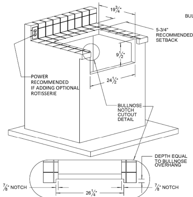
TYPICAL AAEP-26 INSTALLATION
