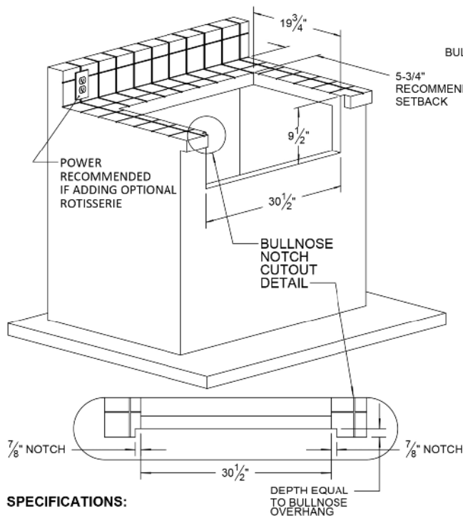
TYPICAL AAEP-32 INSTALLATION
