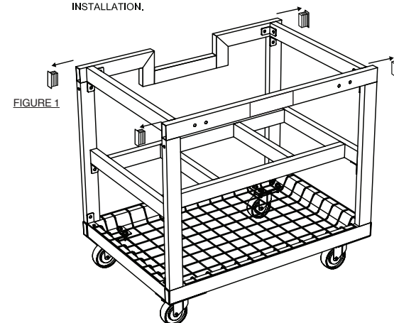
FULLY ASSEMBLED CART
