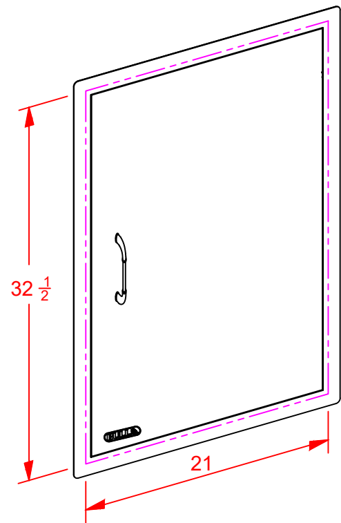
PERSPECTIVE VIEW WITH INSTALLATION CUT OUT DIMENSIONS
