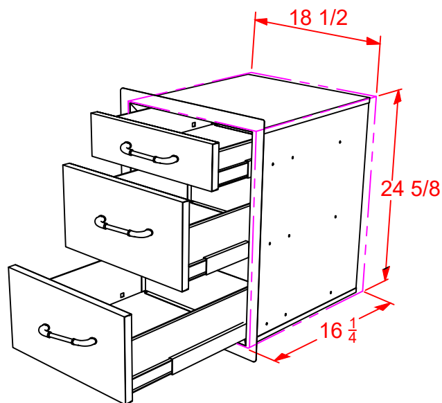
PERSPECTIVE VIEW WITH INSTALLATION CUT OUT DIMENSIONS
