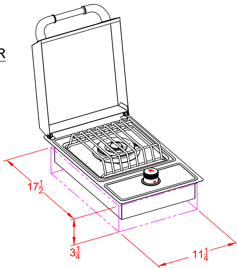
PERSPECTIVE VIEW
