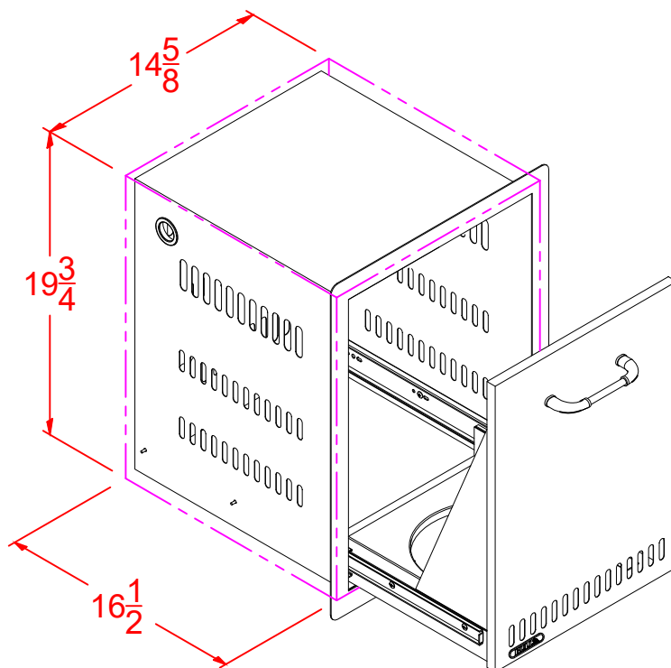
PERSPECTIVE VIEW
