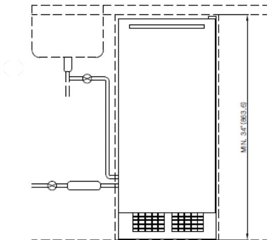
Fig. 7 Front View
