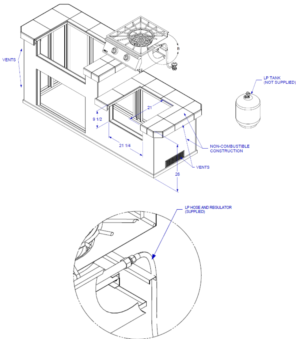
Detail B
