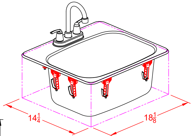
PERSPECTIVE VIEW
