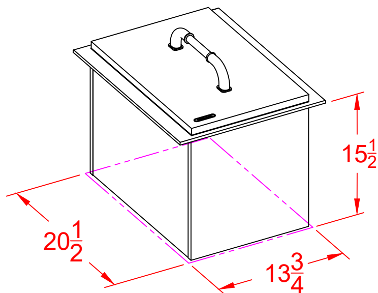
PERSPECTIVE VIEW WITH INSTALLATION CUT OUT DIMENSIONS
