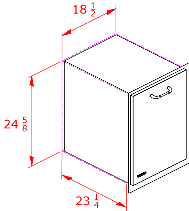
PERSPECTIVE VIEW WITH INSTALLATION CUT OUT DIMENSIONS
