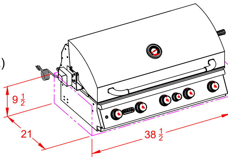
PERSPECTIVE VIEW
