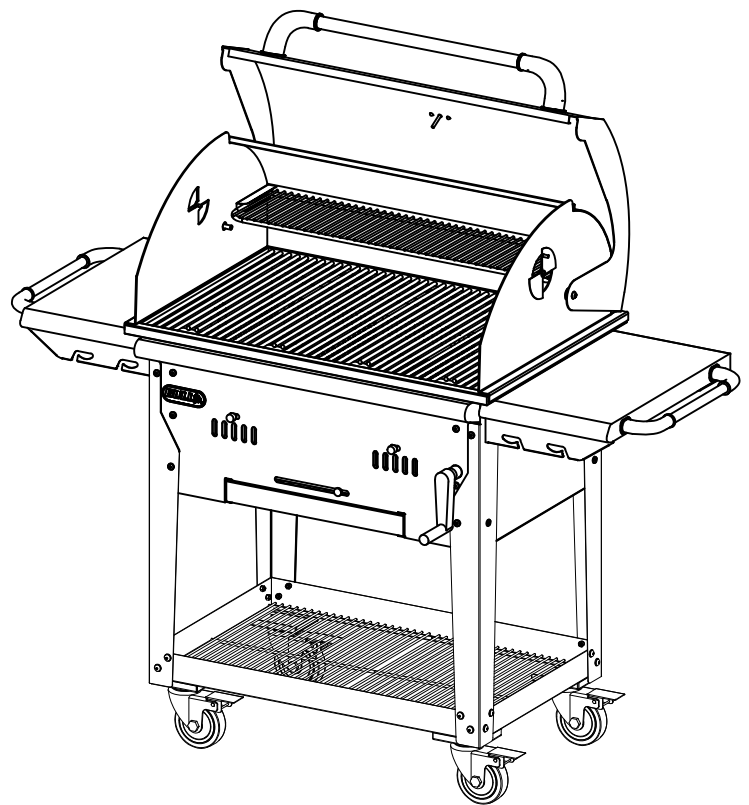
PERSPECTIVE ASSEMBLY VIEW BISON GRILL (SOLD SEPARATELY)
