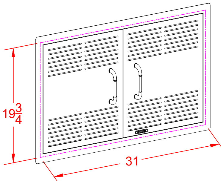
PERSPECTIVE VIEW WITH INSTALLATION CUT OUT DIMENSIONS
