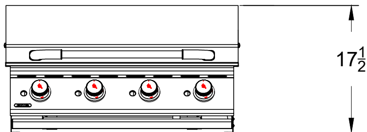
FRONT VIEW
