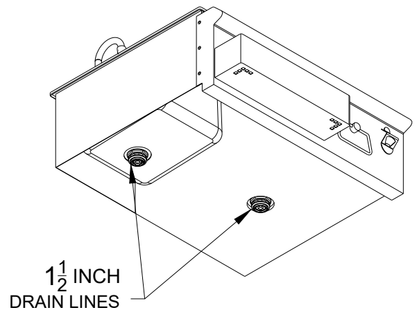
ISOMETRIC BOTTOM VIEW WITH DRAIN LINE DETAILS
