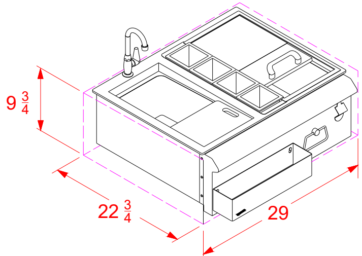
ISOMETRIC TOP VIEW WITH INSTALLATION CUT OUT DIMENSIONS
