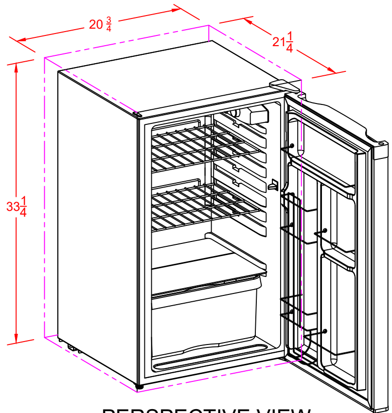
PERSPECTIVE VIEW
